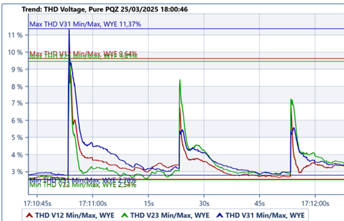
LV side Power Quality recordings – Building #1 UPS upstream
