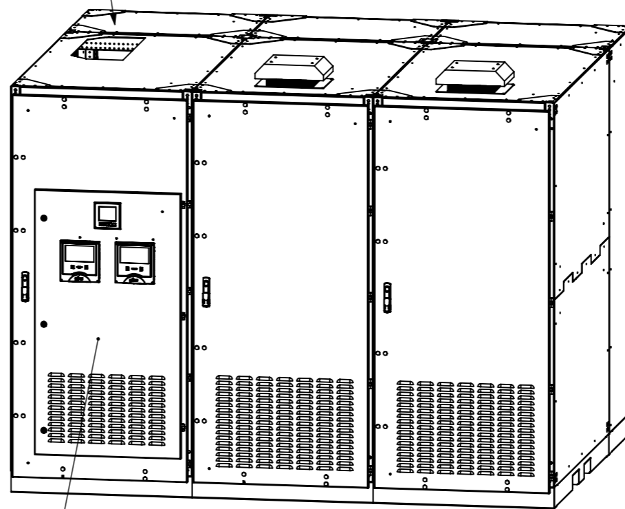
LV cabinet on door
