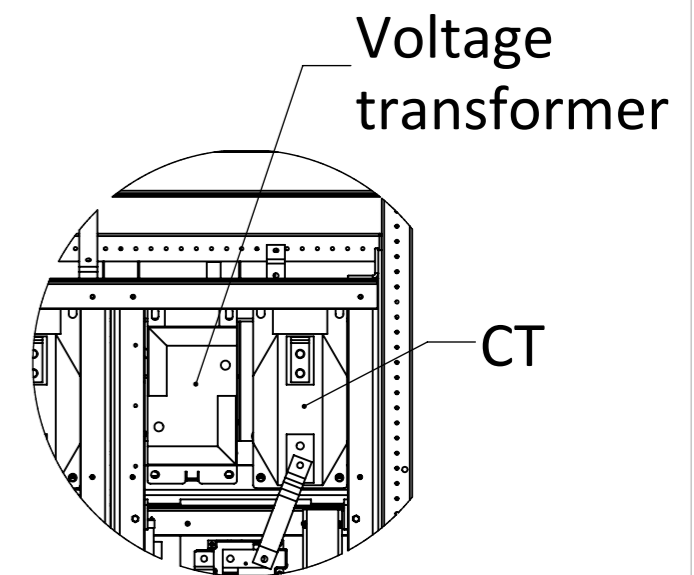
DETAIL J SCALE 2 : 25
